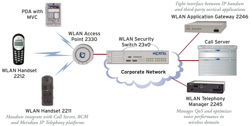
Figure 6. VoWLAN implementation
